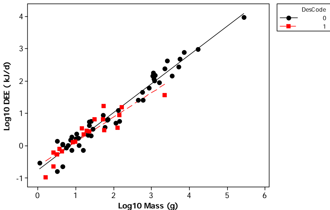
Figure 2. Scatterplot of Log10 DEE vs. Log10 mass indicating data from desert and npn-desert species (DesCode 0 = non-desert, DesCode 1 = desert).
