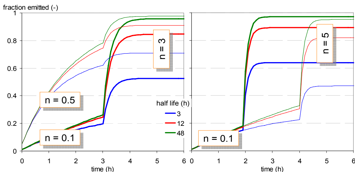
Figure 8. Cumulative emission (as a fraction of the matter present in air after application, not of the applied dose) vs. time, for chemicals having half life of 3 (blue), 12 (red) and 48 (green) hours, respectively, in a number of ventilation scenarios. Left: an air-tight or a leaky greenhouse (0.1 and 0.5 volume exchanges per hour, respectively), open after 3 hours with a ventilation rate of 3 per hour thereafter. Right: an air-tight greenhouse open either after 2 or 4 hours, with a ventilation rate of 5 per hour thereafter. Mean height of the greenhouse is assumed to be 5 m.
