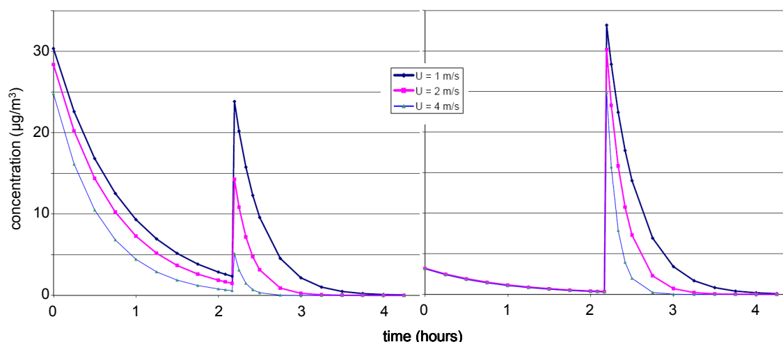
Figure 9. Concentration 20 m leeway of a greenhouse after application of a dose of 1000 g per 3 ha at time = 0. Dutch Venlo glasshouse, left 'leaky' and right well sealed, with three wind speeds. The emission caused by compulsory ventilation (3) is represented by the peak after a bit more than two hours after application. Calculated by Duyzer et al. , 2004, after calibration of the model with measurements.
