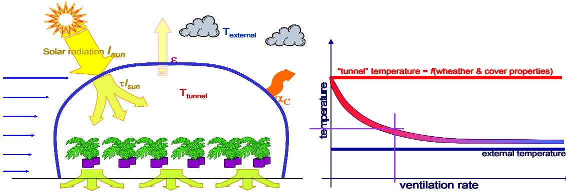
Figure 2. Left: the temperature in an enclosure (tunnel) results from the balance of the energy fluxes in and out of the tunnel. These, in turn, depend on the properties (transmissivity, emissivity and heat transfer) of the cover. Right: the temperature in a ventilated enclosure approaches the external temperature with increasing ventilation rate. Regulated openings adapt the ventilation rate to changing weather, in order to maintain the internal temperature as desired.
