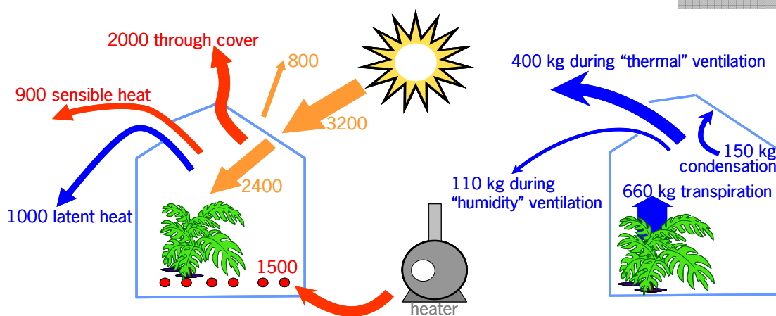
Figure 1. Yearly energy ( \text{MJ m}^{-2} , left) and vapour balance ( \text{kg m}^{-2} , right) of a typical greenhouse in Holland. Ventilation is required to get rid of sun energy (when the greenhouse would become too warm) and also to get rid of water vapour when ventilation would otherwise not be required. Heating is needed to ensure at all times the required temperature whenever sun radiation does not suffice.
